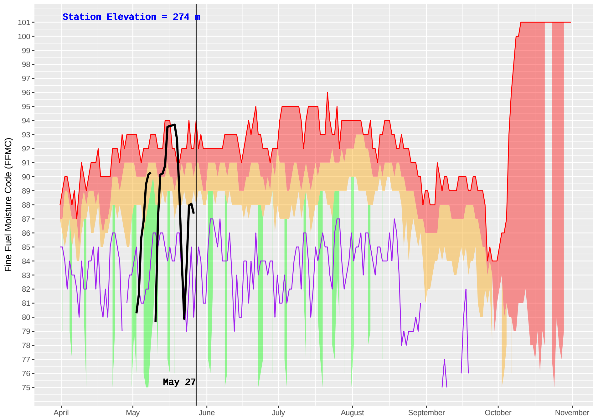
CEDARVALE (429) : Historical (1982–2016) and Current (2018) Noon Fine Fuel Moisture Code (FFMC)
